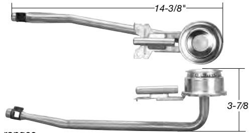
1389 Burner, Rear
