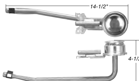
1391 Burner, Rear
